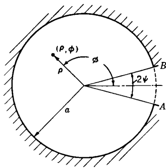
FIG. 2-10.—Cylindrical resonator.
